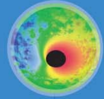
black holes
