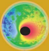
black holes
